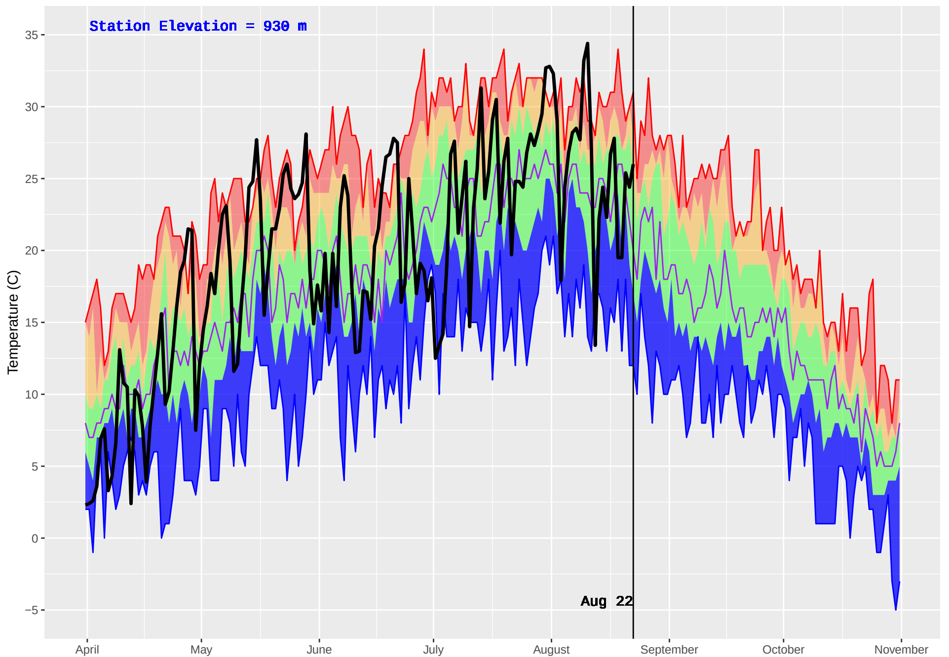
BRISCO (865) : Historical (2004–2016) and Current (2018) Daily Temperature
