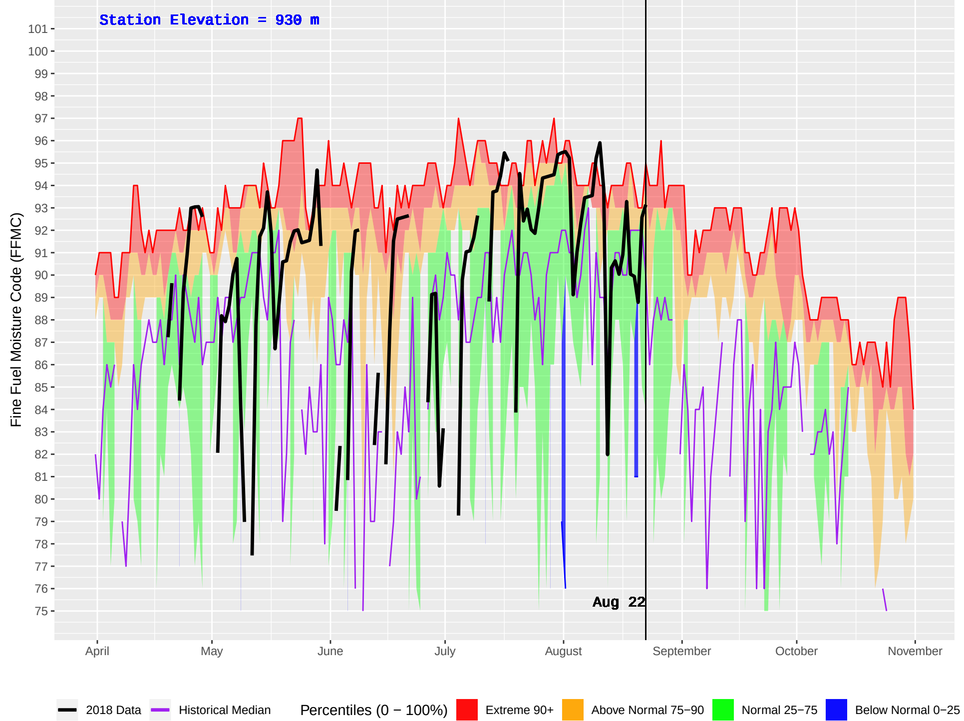
BRISCO (865) : Historical (2004–2016) and Current (2018) Daily Fine Fuel Moisture Code (FFMC)
