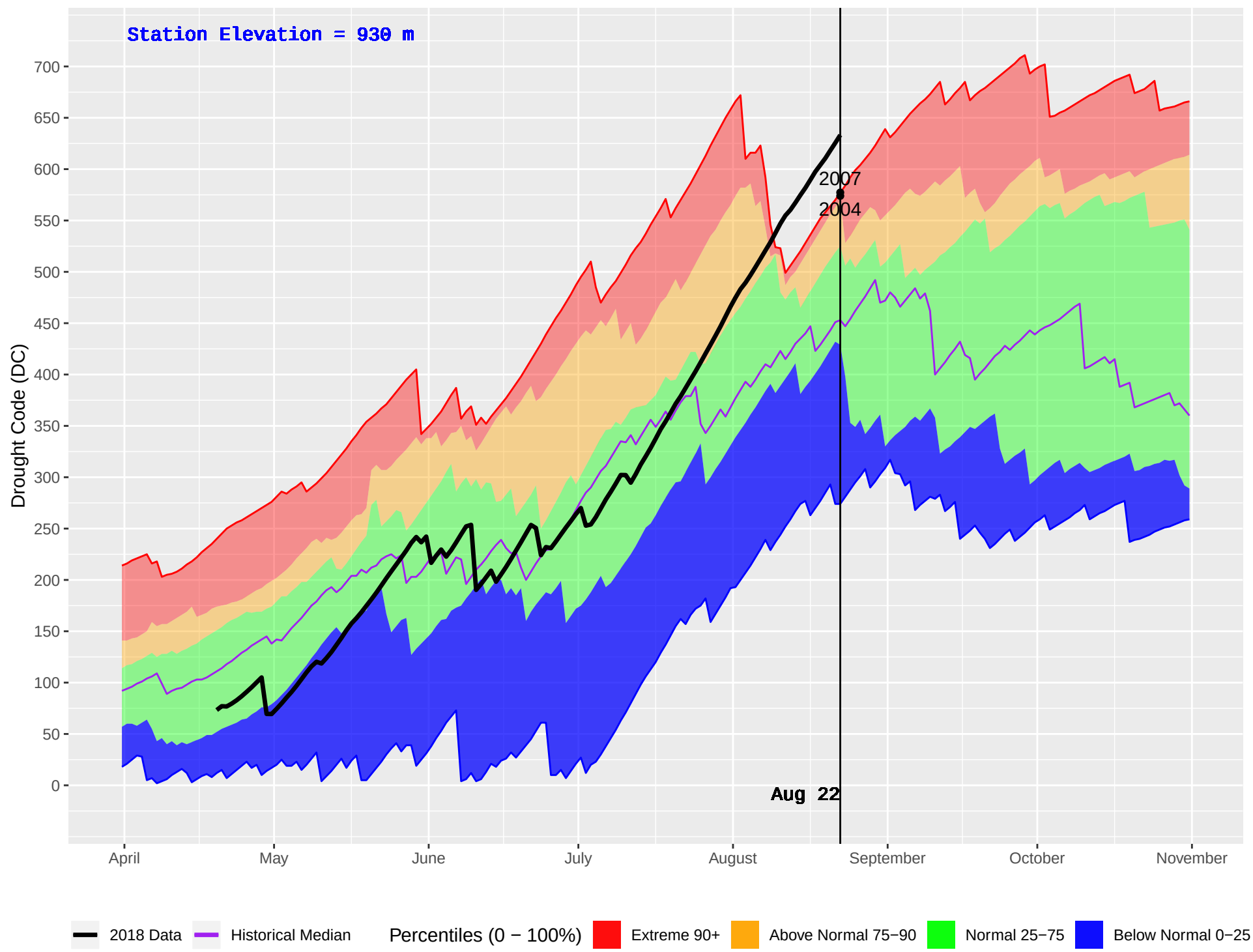
BRISCO (865) : Historical (2004–2016) and Current (2018) Daily Drought Code (DC)
