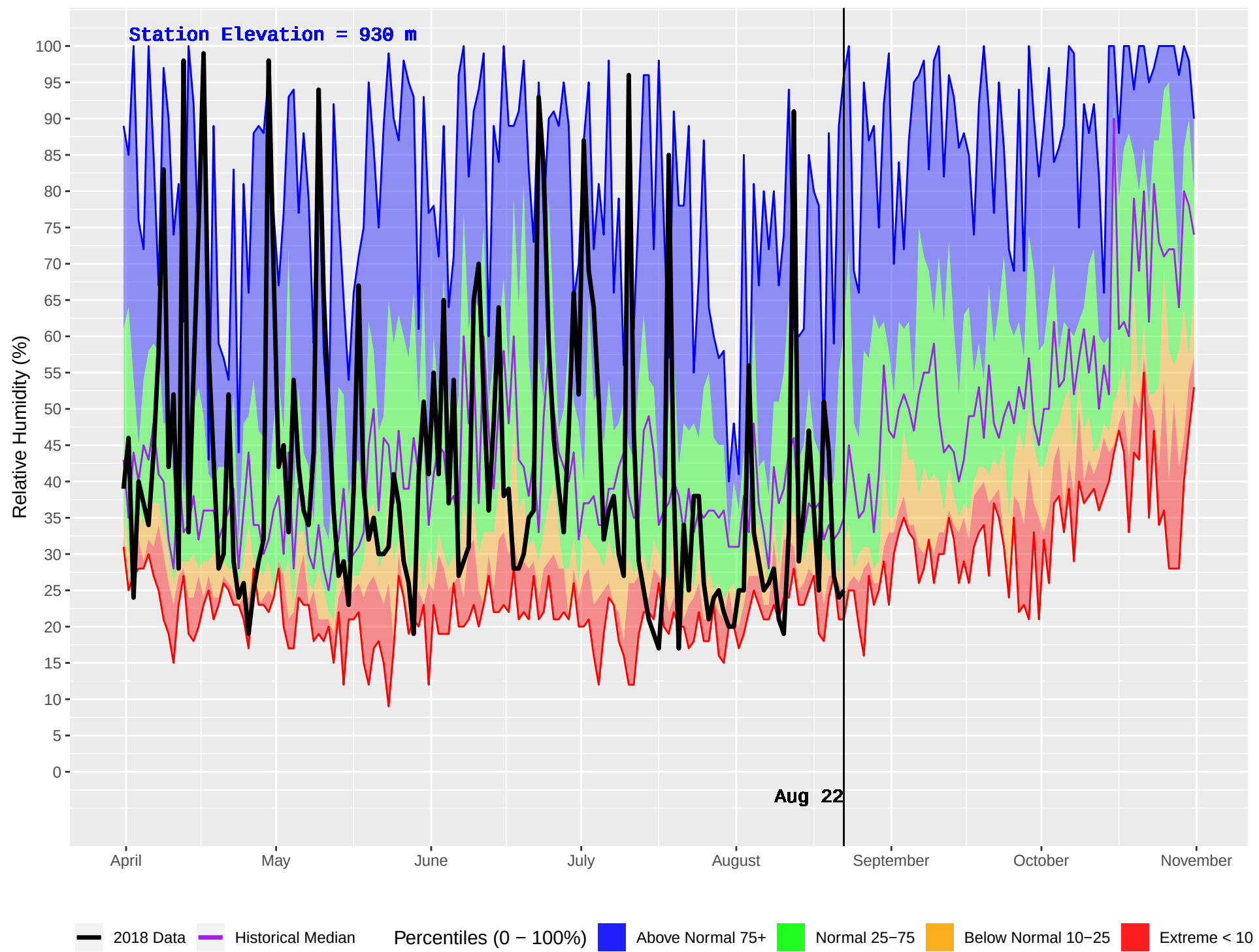
BRISCO (865) : Historical (2004–2016) and Current (2018) Daily Relative Humidity
