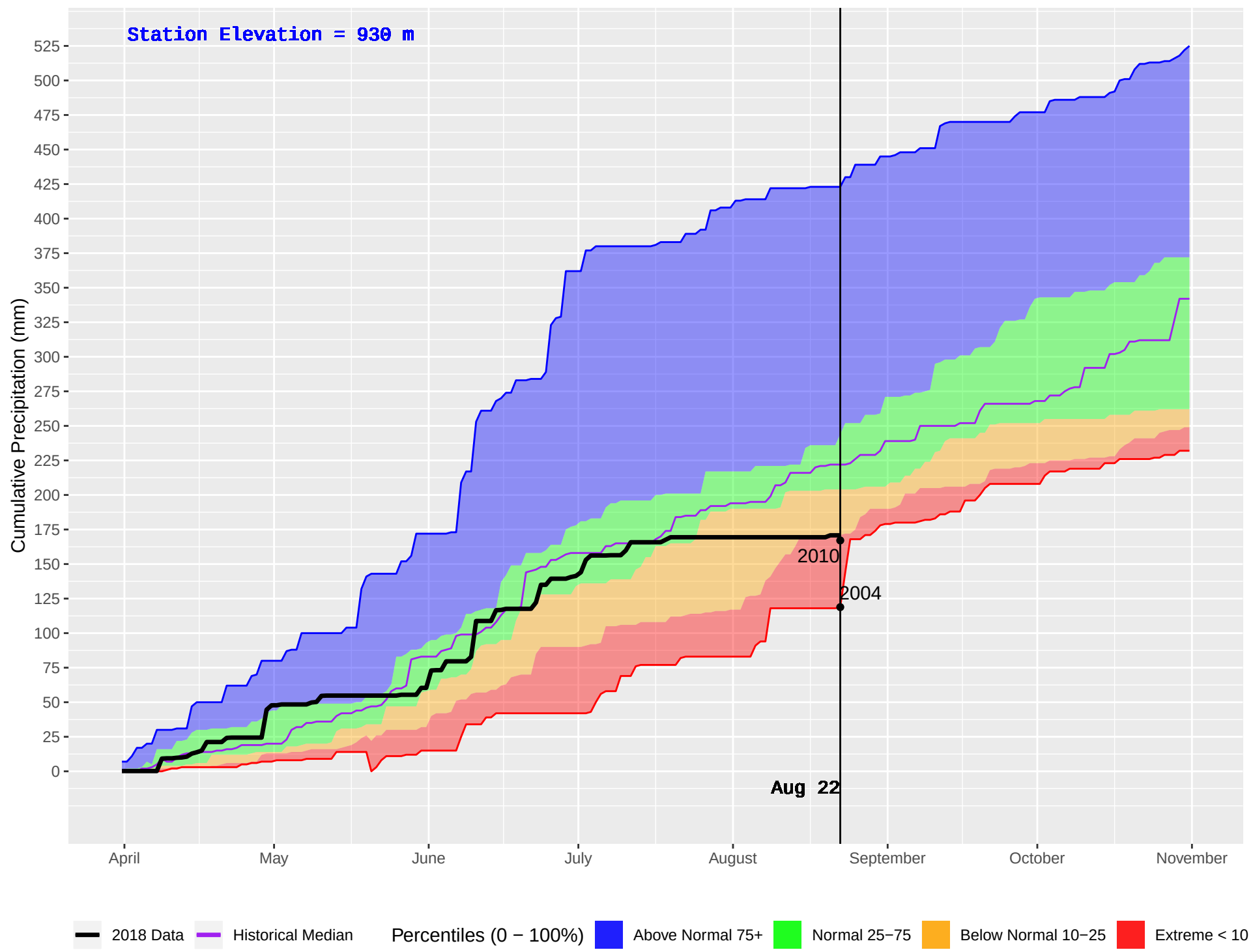
BRISCO (865) : Historical (2004–2016) and Current (2018) Daily Cumulative Precipitation
